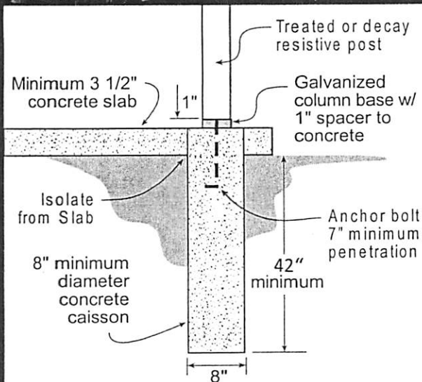
Detail C
